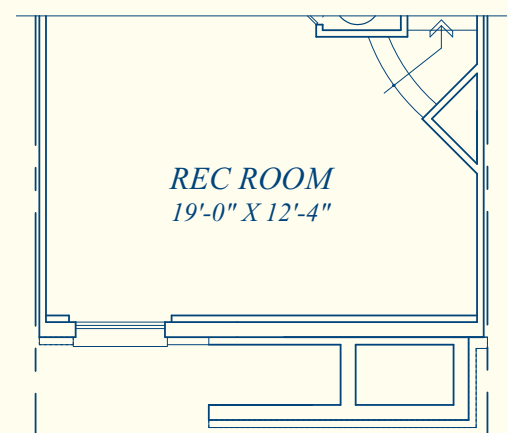
ENGLISH BASEMENT WITH DETACHED GARAGE WITH OPT. 4' EXTENSION (ELEV. #1)
