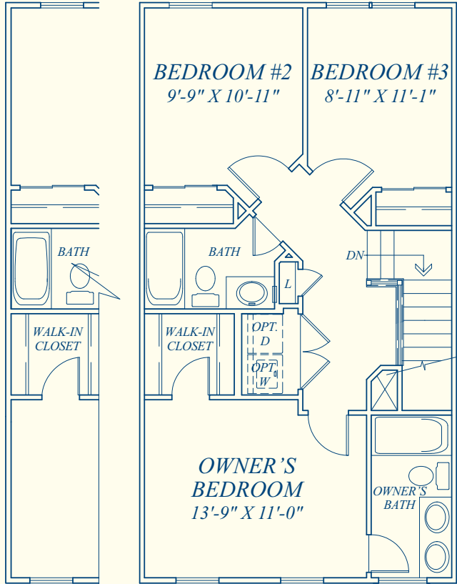
SECOND FLOOR PLAN STANDARD PLAN (SHOWN WITH ELEV. #1)
