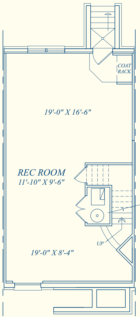
STANDARD PLAN ENGLISH BASEMENT WITH DETACHED GARAGE (ELEV. #1)
