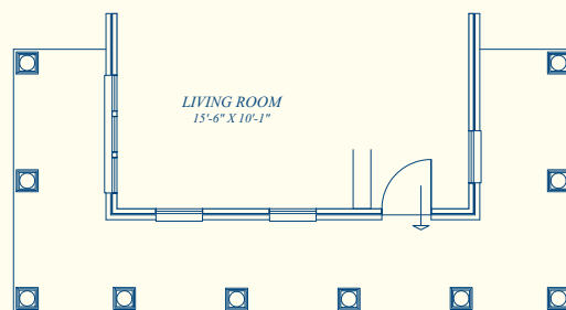
PARTIAL FIRST FLOOR PLAN WITH OPT. WRAP-AROUND PORCH (SHOWN WITH ELEV. 2, AVAILABLE WITH ELEV. 6)
