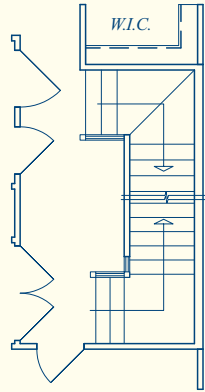
STAIRS AT OPT. LOFT BEDROOM**
