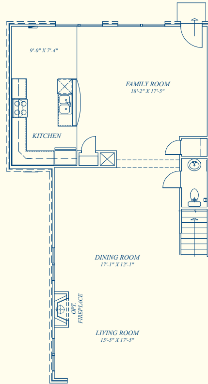
PARTIAL FIRST FLOOR PLAN WITH OPT. DETACHED GARAGE
