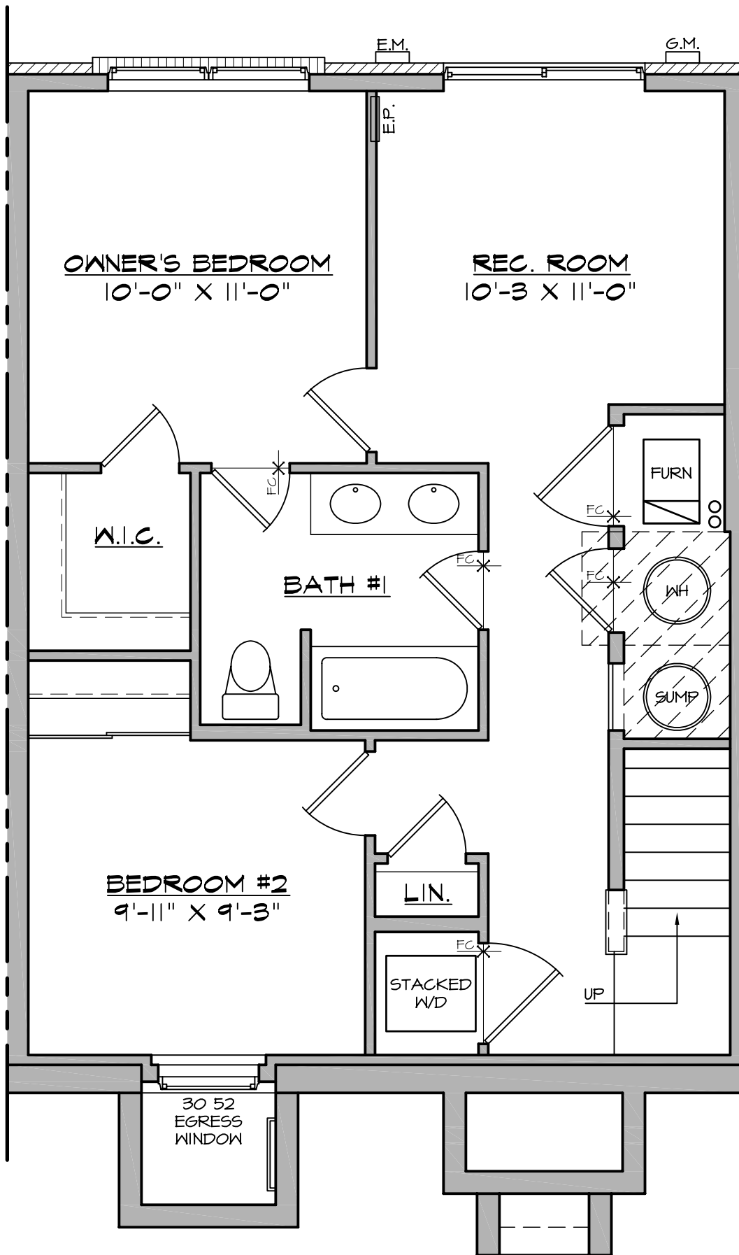
JAMES MODEL FIRST FLOOR PLAN
