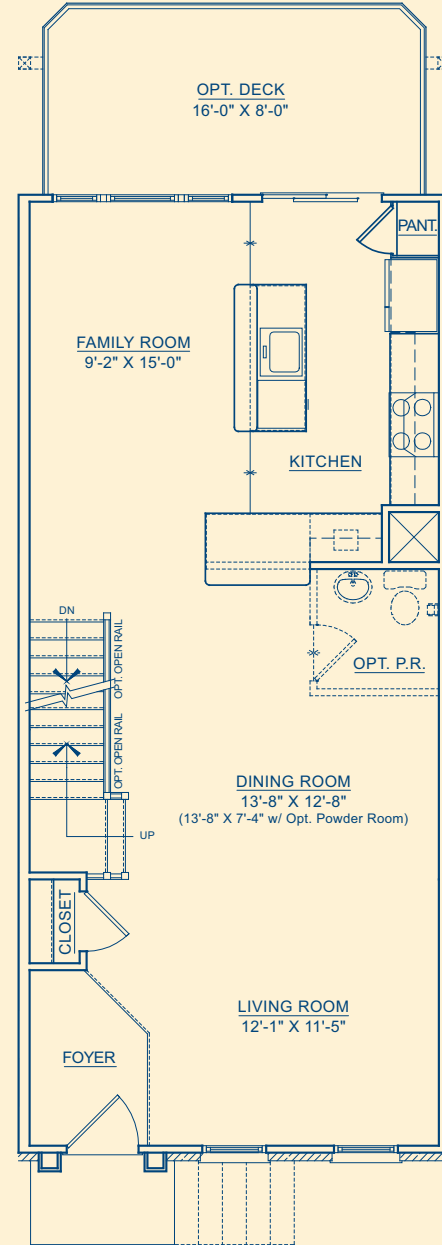
OPTIONAL BURIED OR ENGLISH FRONT
