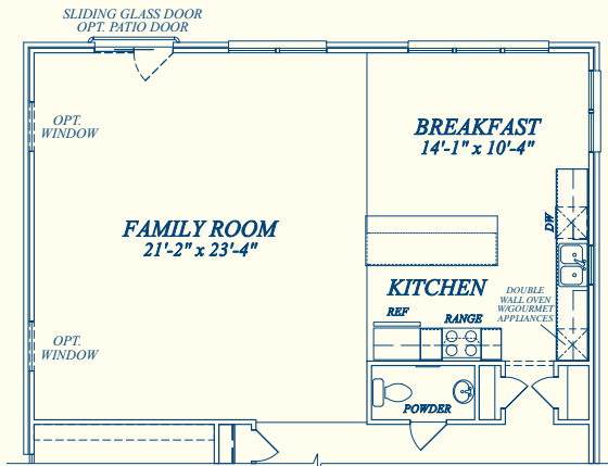
FIRST FLOOR PLAN W/EXT. FAMILY ROOM W/ OPT. ENGLISH BASEMENT
