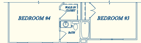
SECOND FLOOR PLAN PARTIAL (SHOWN WITH ELEV. 3)
