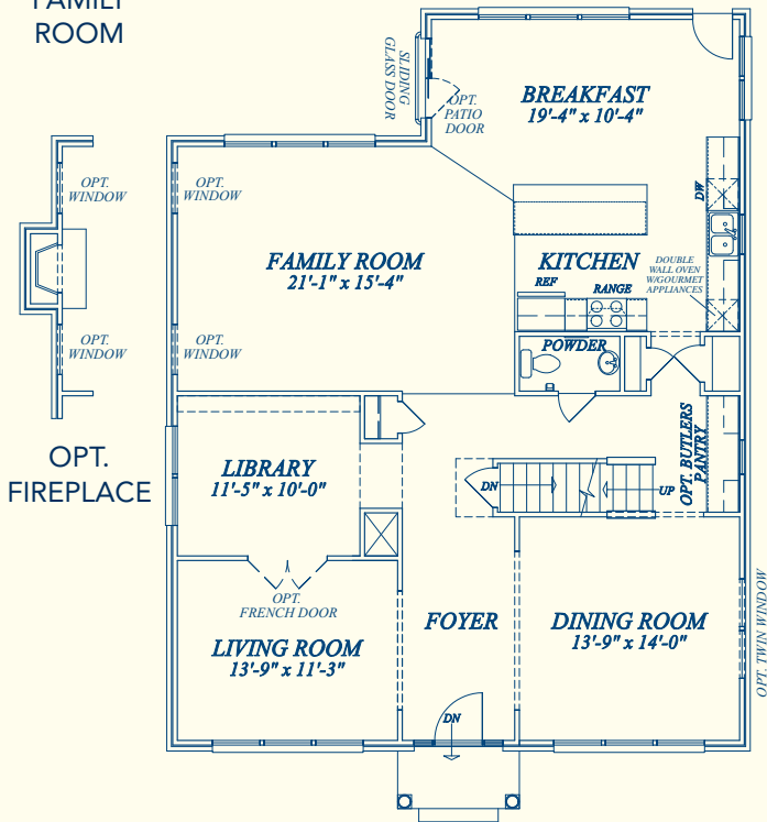
OPT. FIREPLACE W/EXT. FAMILY ROOM FIRST FLOOR PLAN W/EXT. FAMILY ROOM W/CRAWL SPACE
