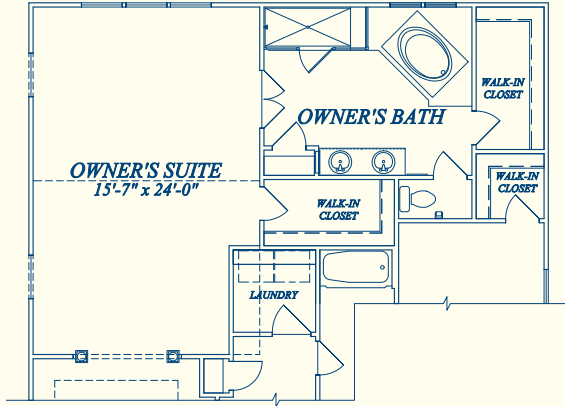
SECOND FLOOR PLAN W/ OPT. EXT. MASTER BEDROOM
