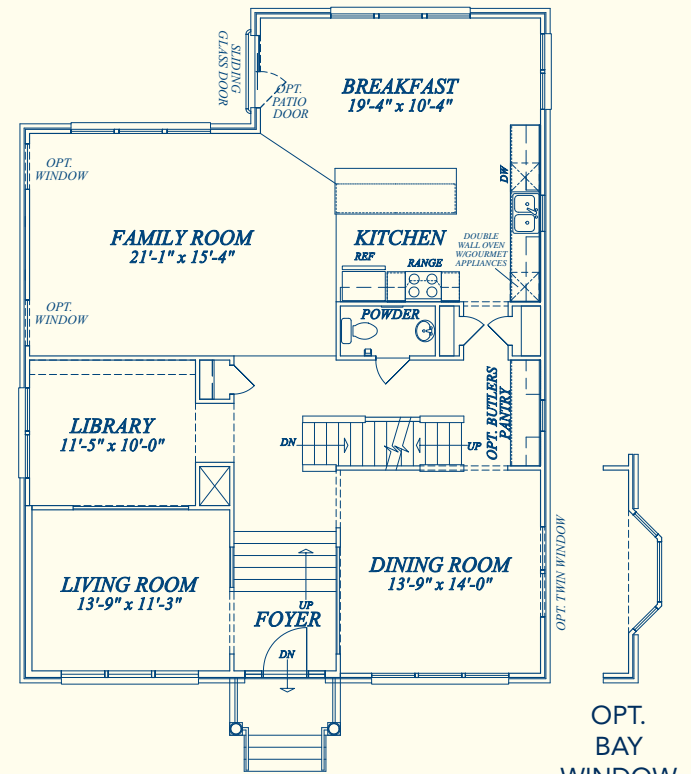
FIRST FLOOR PLAN W/ OPT. ENGLISH BASEMENT (SHOWN WITH ELEV. 1)
