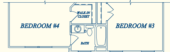
SECOND FLOOR PLAN PARTIAL (SHOWN WITH ELEV. 2)
