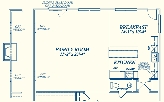
OPT. FIREPLACE W/EXT. FAMILY ROOM FIRST FLOOR PLAN W/EXT. FAMILY ROOM W/CRAWL SPACE
