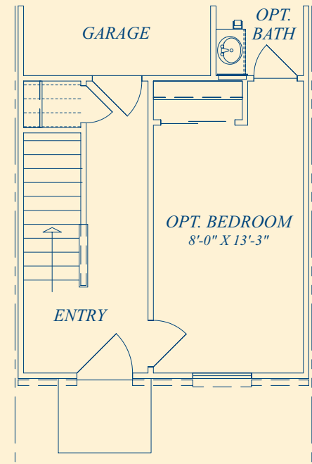
PARTIAL LOWER LEVEL PLAN W/ OPT. BEDROOM
