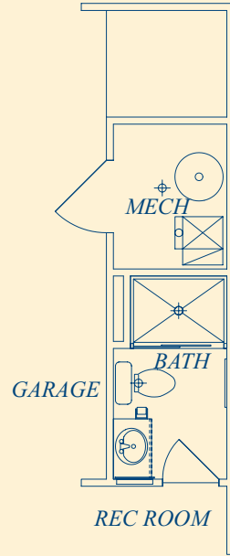
PARTIAL LOWER LEVEL PLAN W/ OPT. BATH
